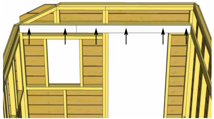
Front Walls
