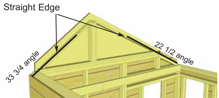
Triangular Gable Trim attached in Step 63.
