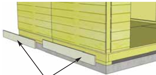
2 pieces of Bottom Skirting per side
