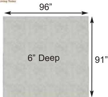
Shed Front
