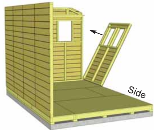
21. Front Side Wall Panel will sit flush with floor framing in corner when positioned correctly. Position Right Side Double Window Wall on floor.
