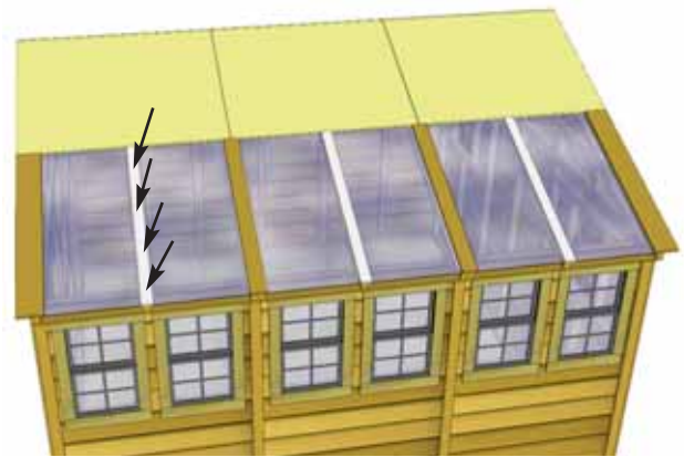
76. Position and attach Mid Ridge Caps, evenly spaced on mid rafters. Align top to bottom as per Step 74.
