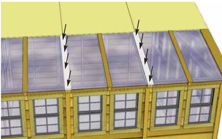
77. Align and attach remaining Ridge Caps (4 1/2" wide) over Double Rafters as per Step 74.
