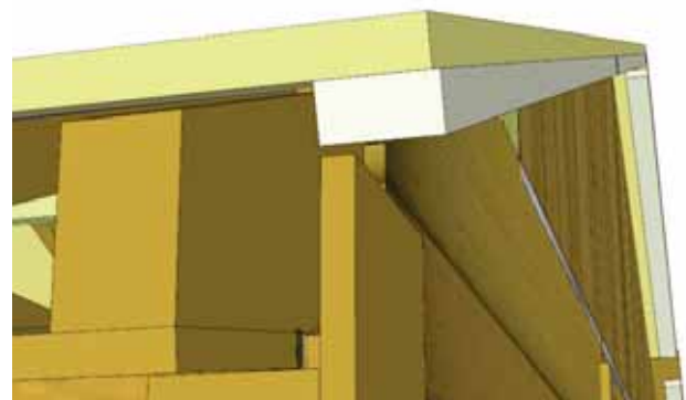
78. Attach Facia Cleat (3/4" x 1 1/2" x 36 1/2") centered on underside of Short Roof plywood, flush to edge. Attach Facia Cleats (3/4" x 1 1/2" x 40") to underside of Long Roof plywood, 1/2" from ends and flush to edge. Repeat this step on the rear side of shed. Fasten with 3 - 1 1/4" screws per piece.
