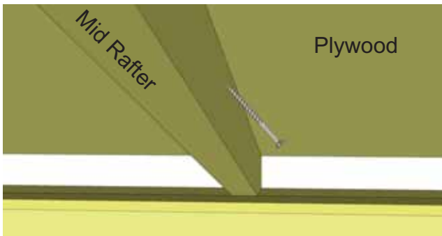
3 - 2 1/2" screws Toe Nailed in each Mid Rafter.
