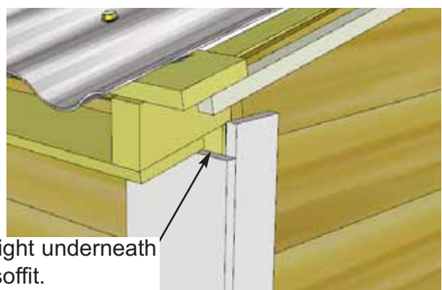
60. To completely trim out rear corners, locate Side Rear Corner Trims (1/2" x 2 1/2" x 80") and Rear Corner Trims (1/2" x 5 1/2" x 79"). Align and attach as per Step 59.
