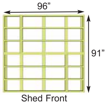
Floor Frame
